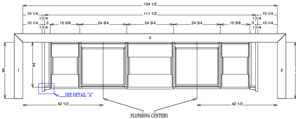
6.12 MASTER BATH VANITY PLAN 5 Scale: 1/2" = 1'
