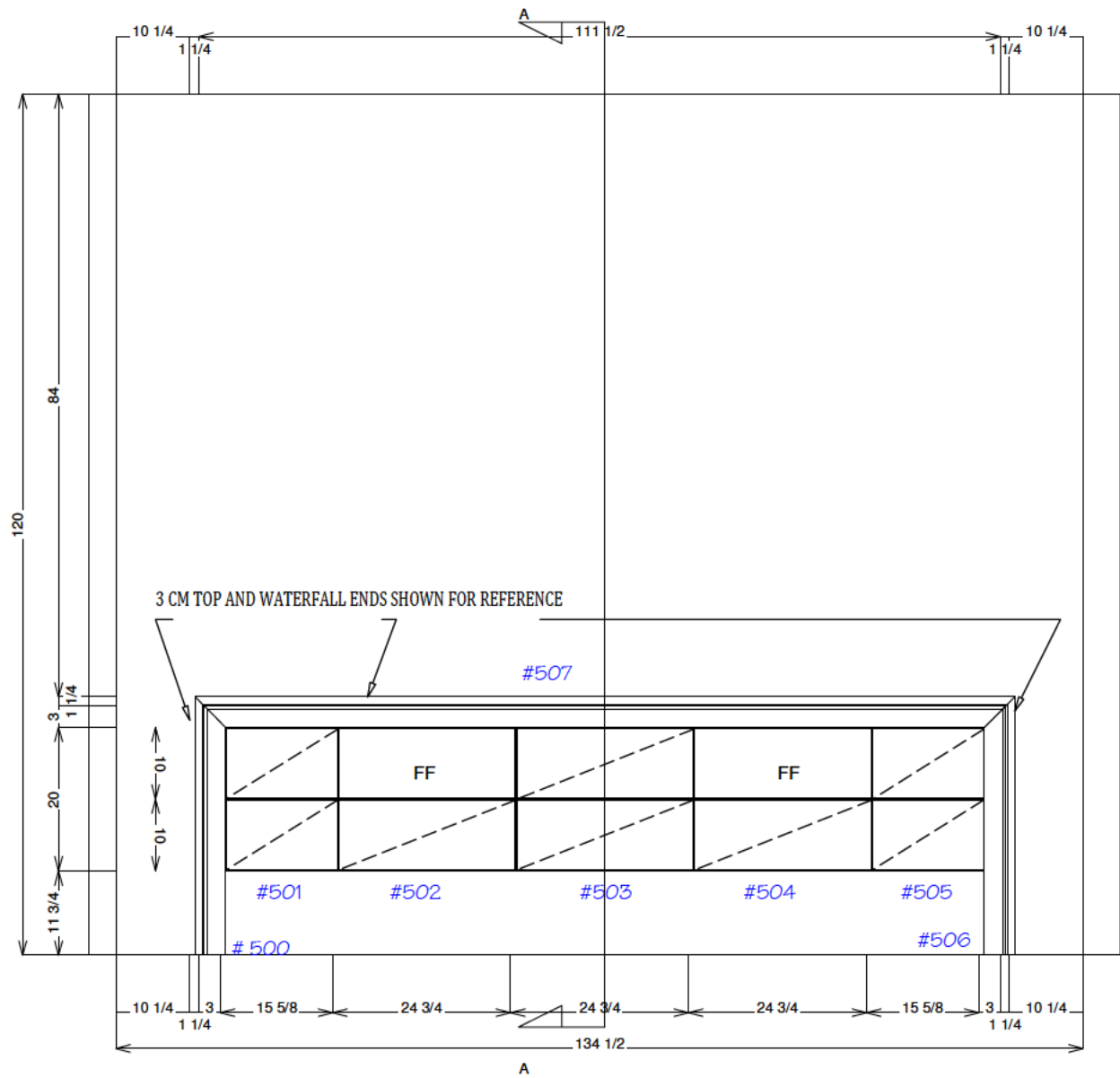
6.12 MASTER BATH VANITY ELEVATION Scale: 1/2" = 1'
